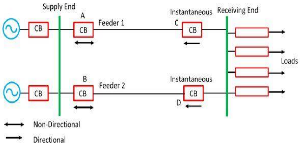
Fig. 3 Protection of Parallel Feeders
