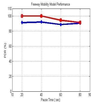
Figure 14. PDR of Freeway
