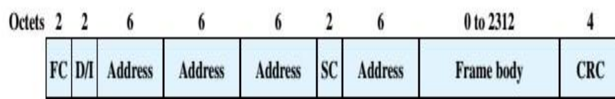
Figure 2. IEEE 802.11 Mac Frame Format
