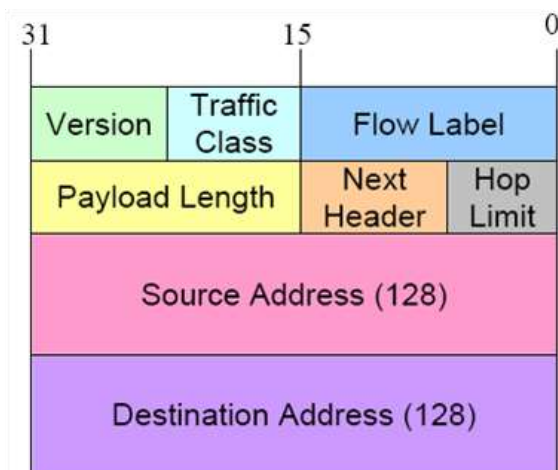
Figure 3. An IPv6 Header Format
