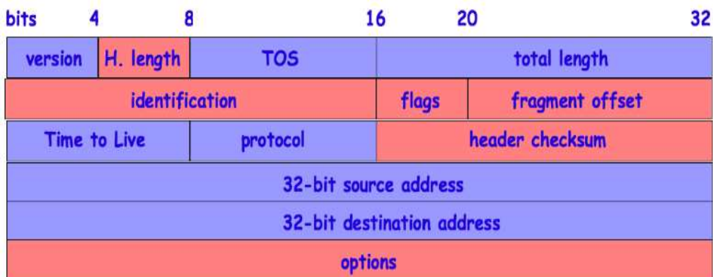
Figure 2. An IPv4 Header Format
