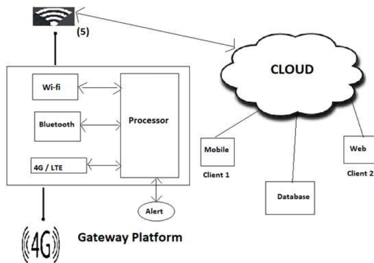
Fig.2 BLOCK DIAGRAM OF MASTER CIRCUIT
