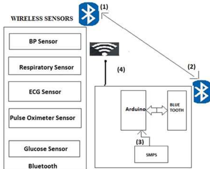
Fig.1 BLOCK DIAGRAM OF SLAVE CIRCUIT
