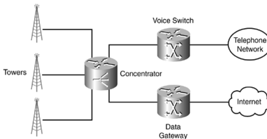
Fig 5 Wireless Wide Area Network [12]
