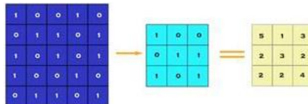
Fig. 2. Convolution of 5 \times 5 image with 3 \times 3 filter image pixel (stride = 1 \times 1 pixel)
